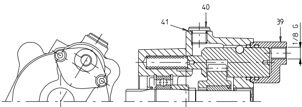
DETAIL PNEUMATIC SHIFTING
