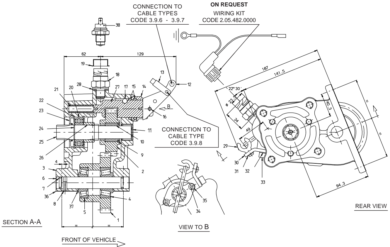
DETAIL PNEUMATIC SHIFTING
